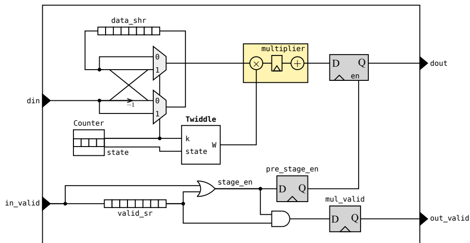
Figure 3.12: Inside a single R2SDC Stage. All modules with wedge is clocked
