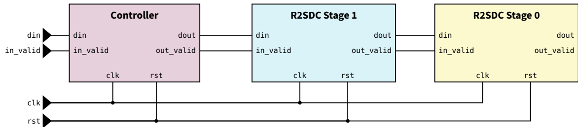
Figure 3.11: Schematic of R2SDC implementation
