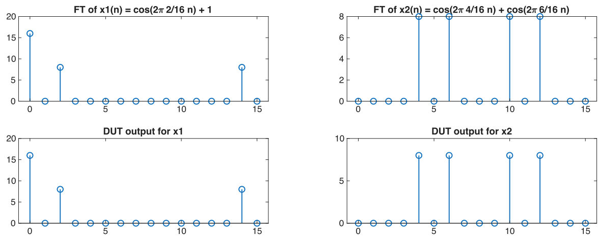
Figure 3.17: Comparison of output of FFT in MATLAB and simulation
