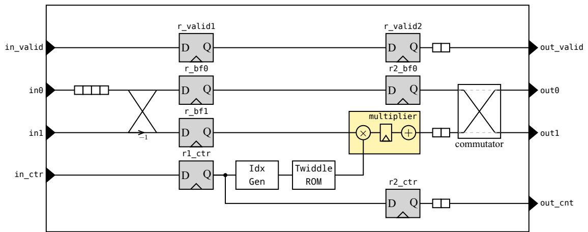
Figure 3.9: Inside a single R2MDC Stage. All modules with wedge is clocked
