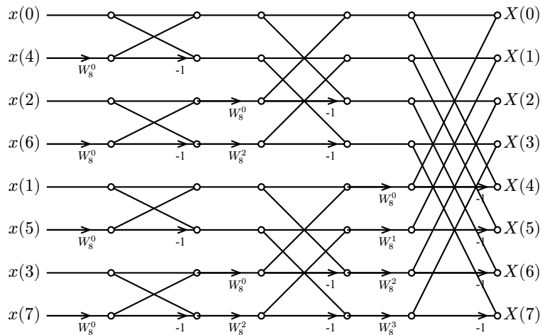
Figure 3.2: Signal flow graph of 8-point radix-2 DIT-FFT
