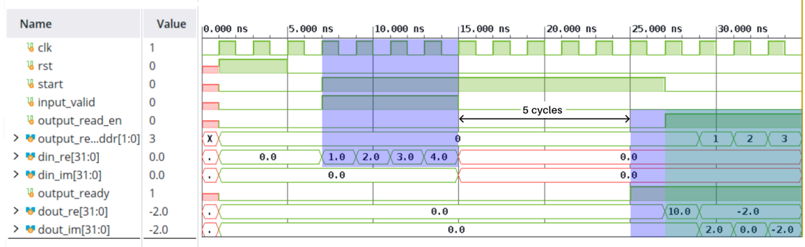
Figure 3.5: Simulation result of 4 point Radix-2 DIT-FFT for a ramp input
