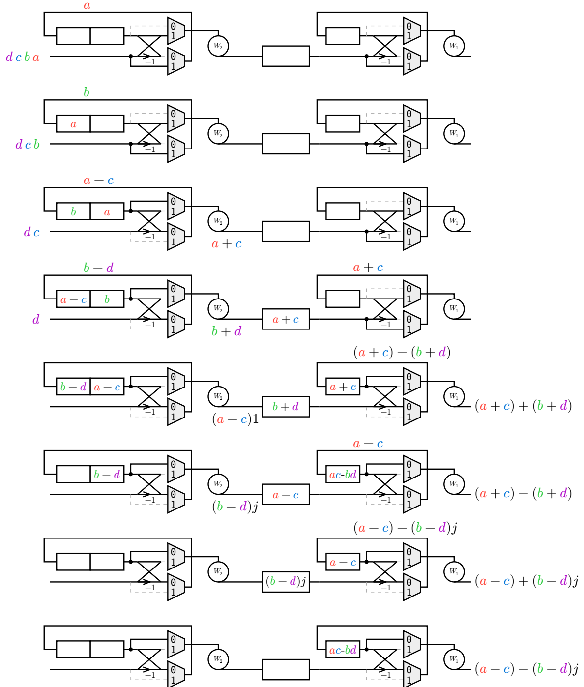
Figure 3.13: Steps involved in a 4 point R2SDC algorithm
