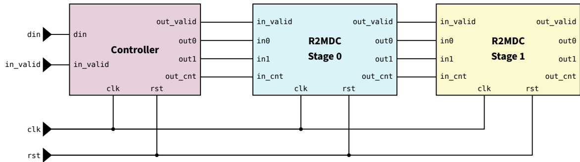
Figure 3.8: Schematic of R2MDC implementation
