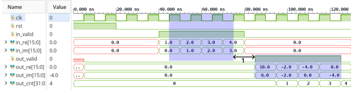
Figure 3.14: Simulation result for 4 point complex test signal in R2SDC
