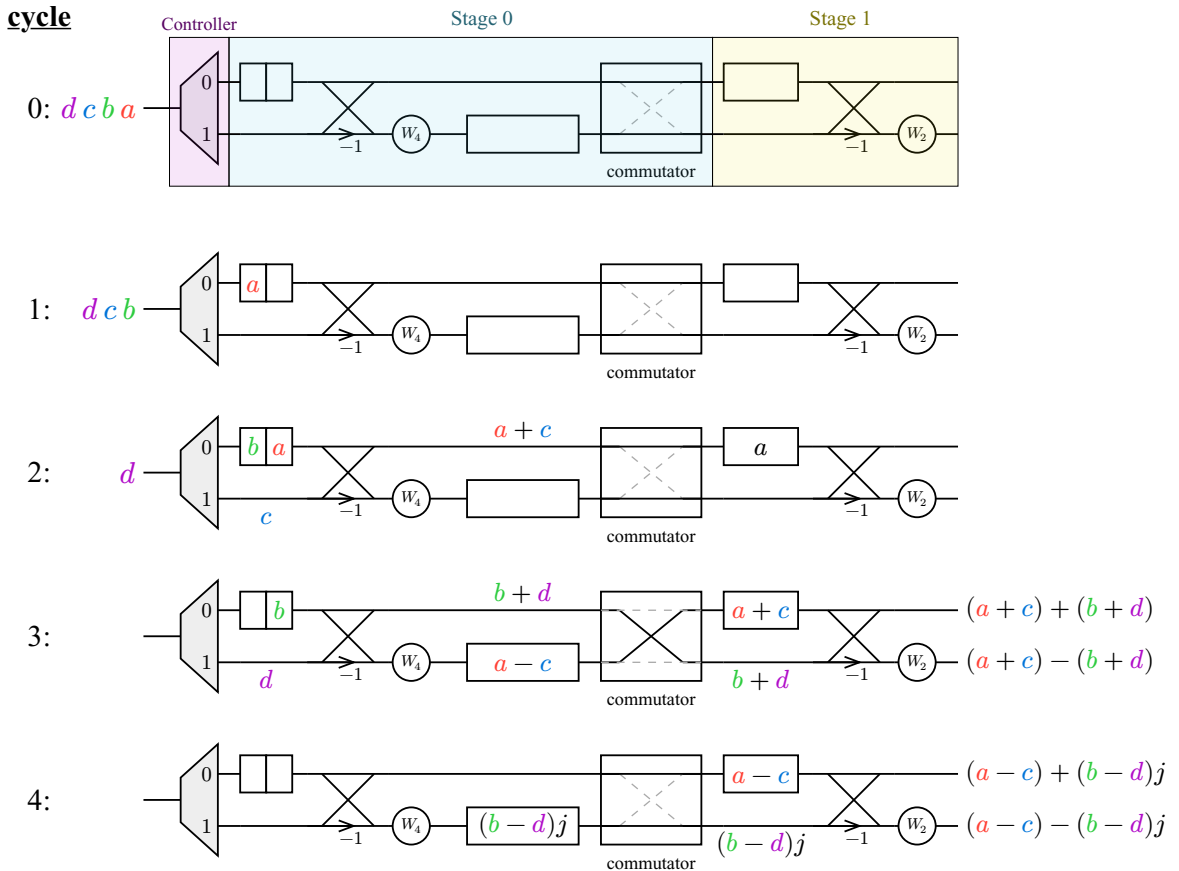
Figure 3.7: Steps in R2MDC algorithm for 4 point case
