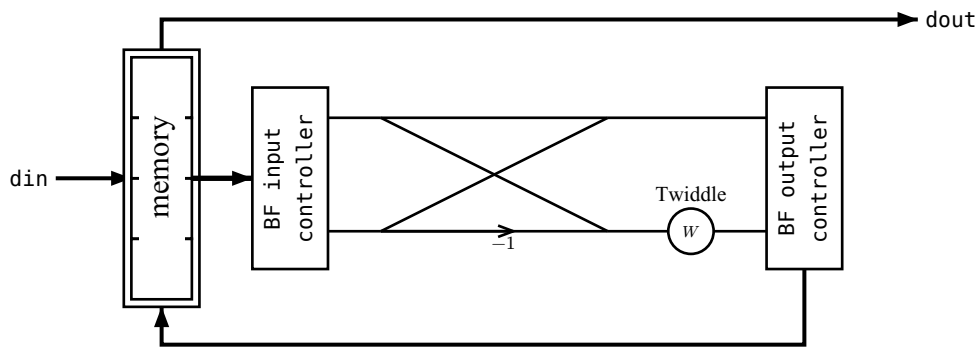
Figure 3.3: Circuit of Radix-2 In-place implementation
