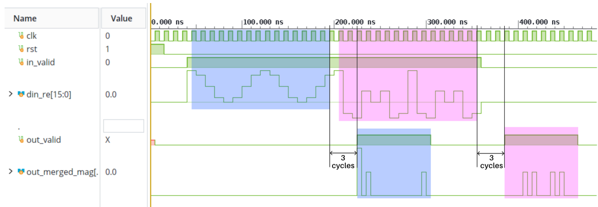
Figure 3.16: Output of 16 point 4-stage pipelined Winograd implementation for 2 consecutive inputs.
