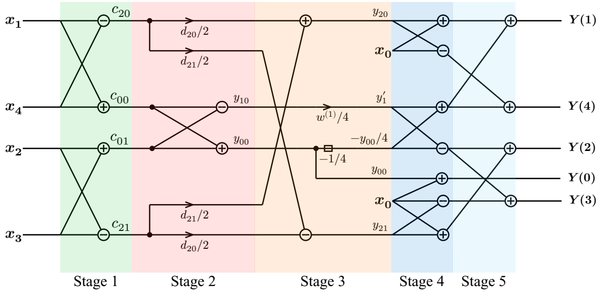
Figure 3.15: Signal flow of modified Winograd algorithm for 5 point DFT.
