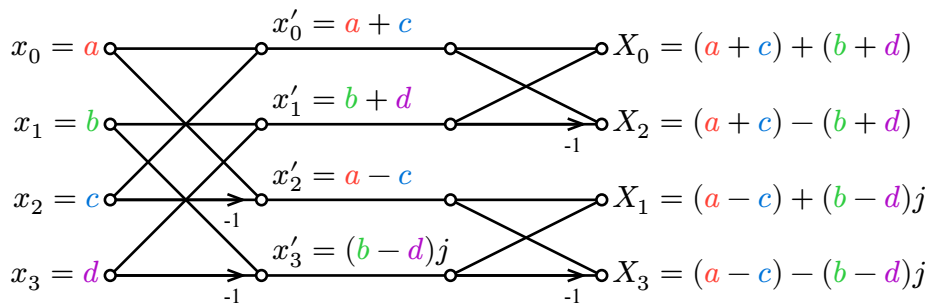
Figure 3.6: Signal flow graph of 4-point radix-2 DIF-FFT
