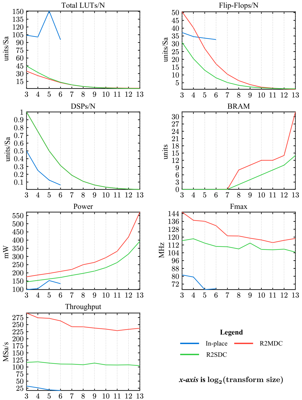
Figure 4.1: Resource and performance analysis of scalable techniques.
