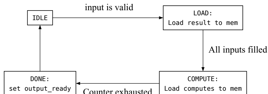
Figure 3.4: Working of FSM in Radix-2 DIT FFT
