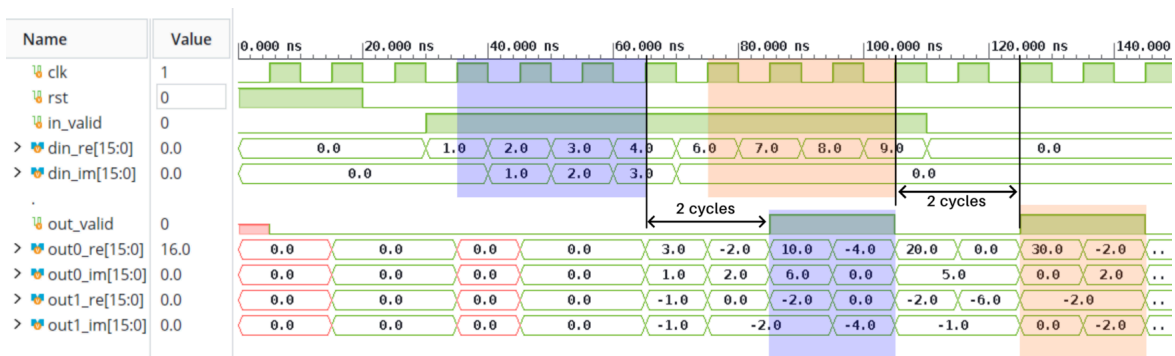
Figure 3.10: Simulation result for two 4 point test signals in R2MDC
